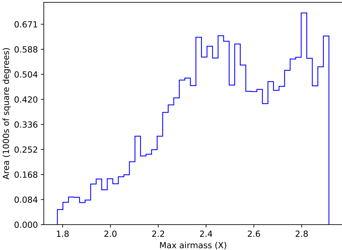
internal_u_expt27_nscale1.0v3.4_10yrs WFD z band: Max airmass
