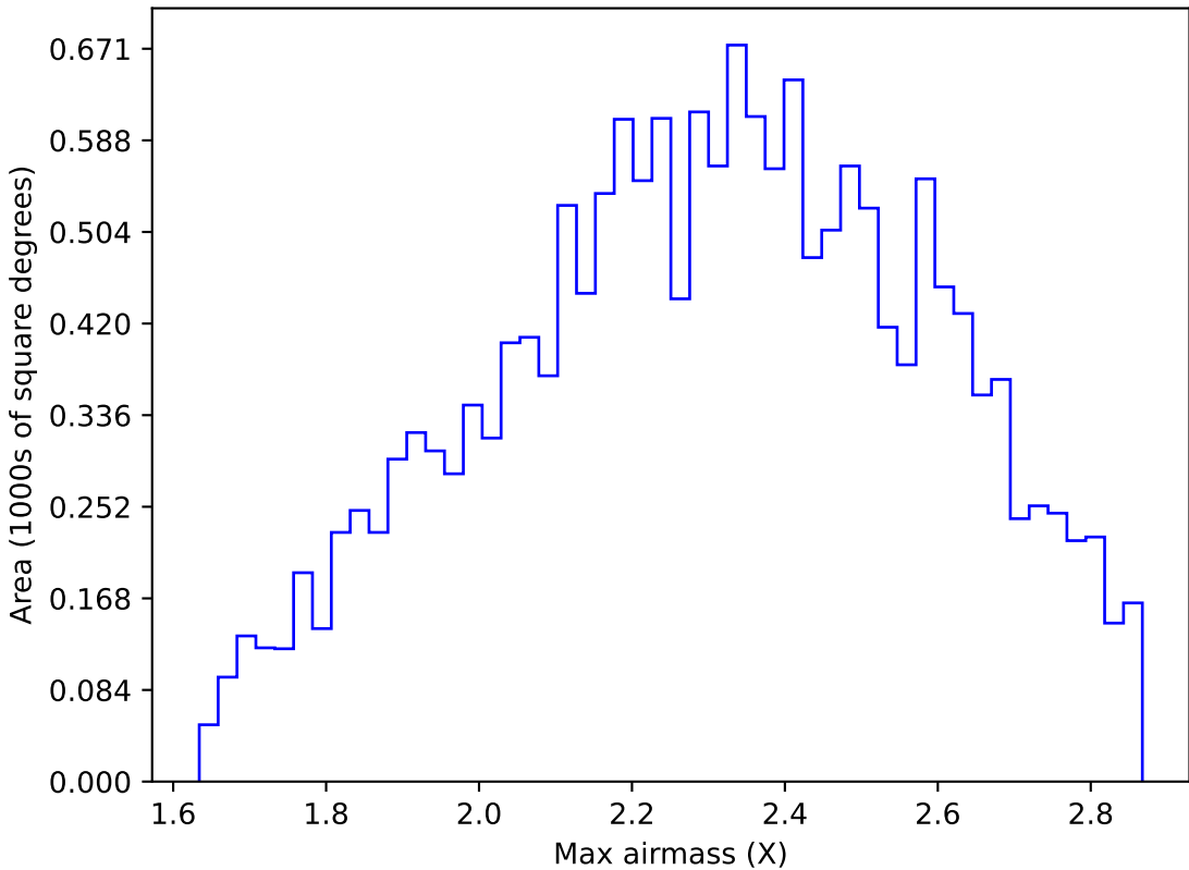
internal_u_expt27_nscale1.0v3.4_10yrs WFD y band: Max airmass
