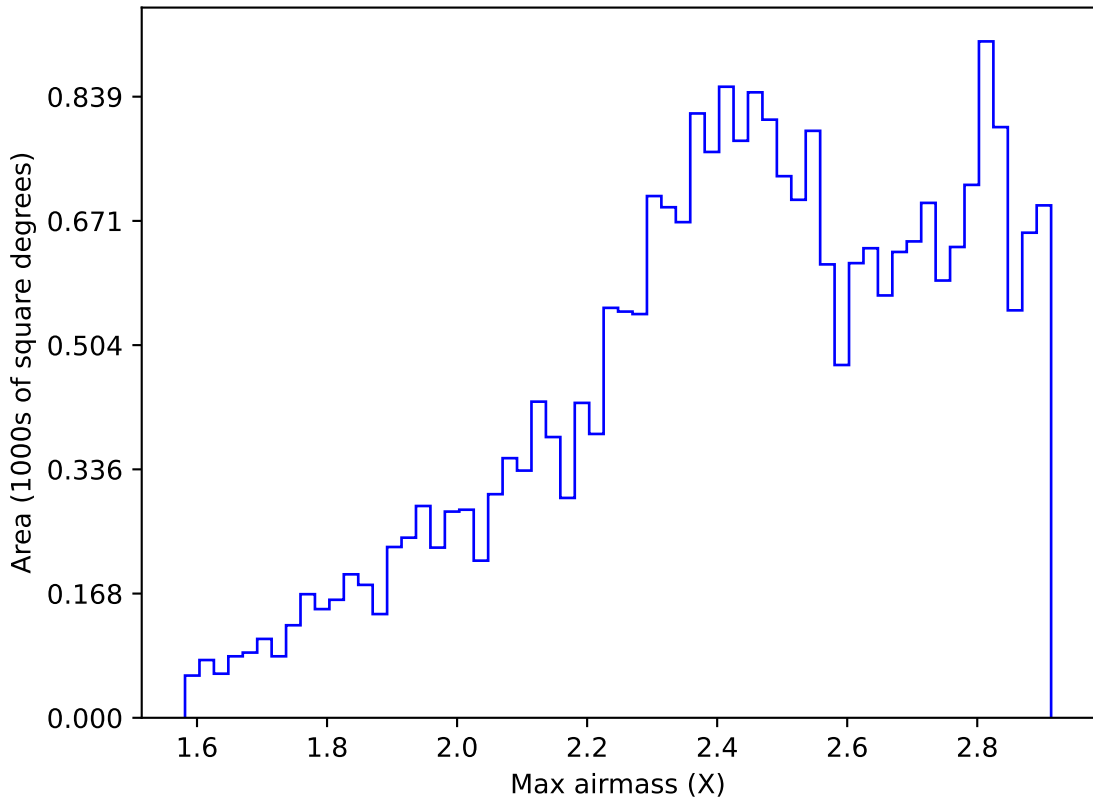
internal_u_expt27_nscale1.0v3.4_10yrs All sky z band: Max airmass
