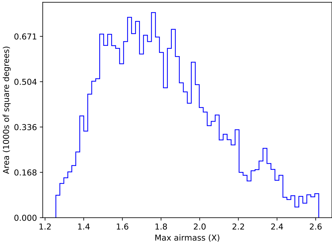
internal_u_expt27_nscale1.0v3.4_10yrs All sky u band: Max airmass
