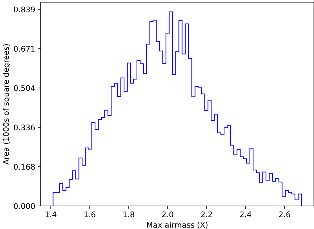
internal_u_expt27_nscale1.0v3.4_10yrs All sky g band: Max airmass
