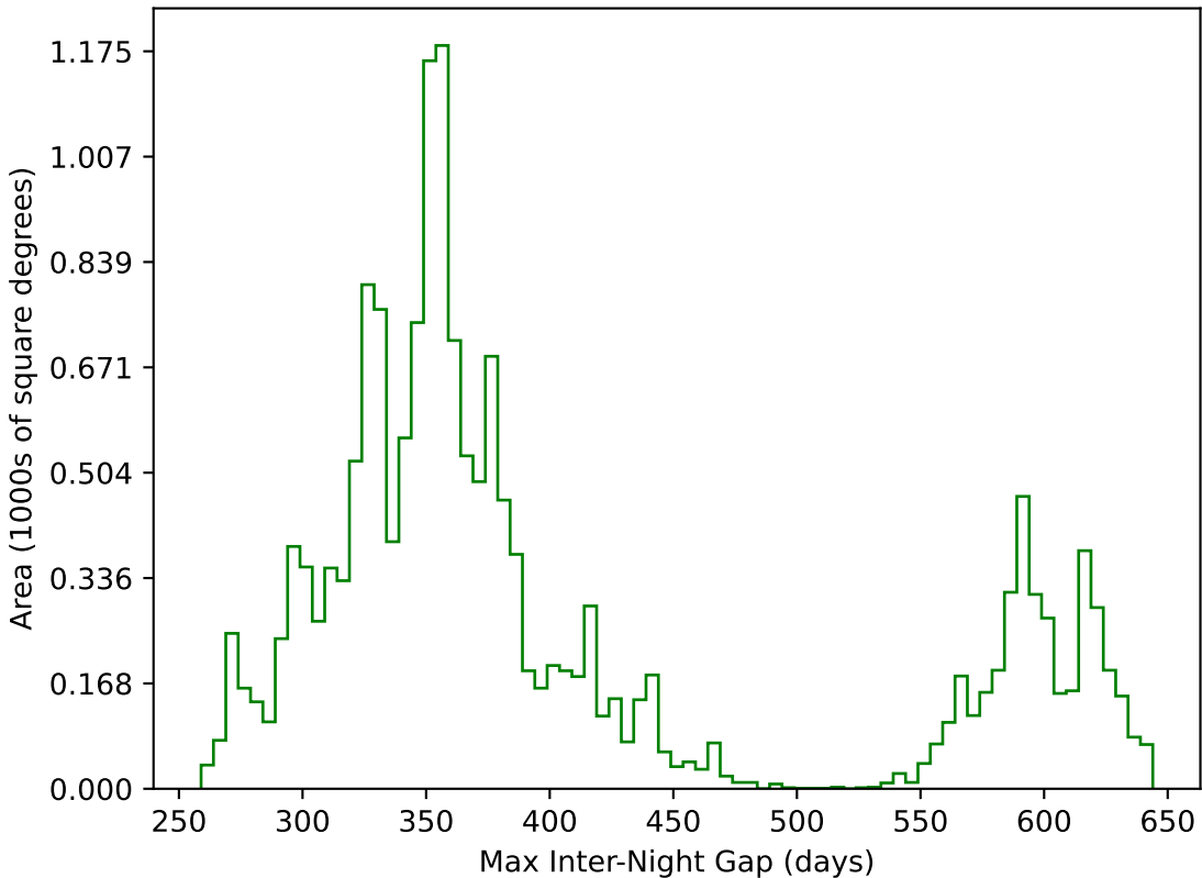
internal_u_expt27_nscale1.0v3.4_10yrs WFD g band: Max Inter-Night Gap
