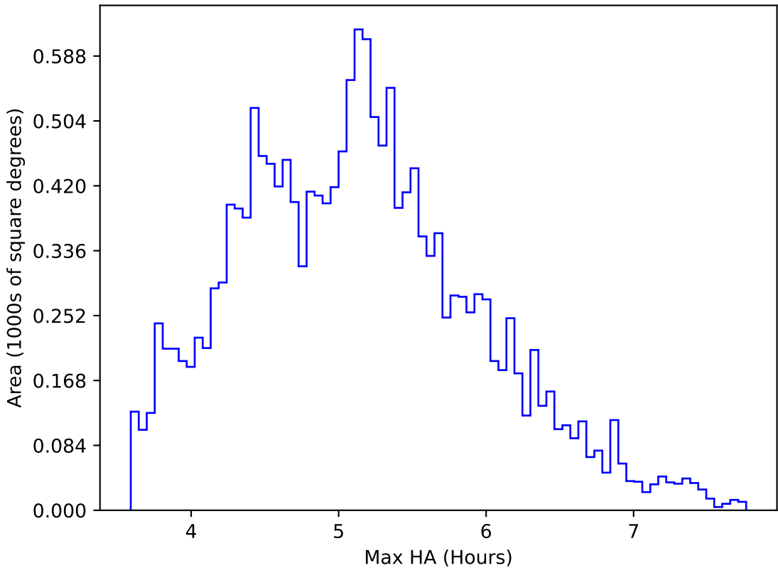
internal_u_expt27_nscale1.0v3.4_10yrs WFD all bands: Max HA
