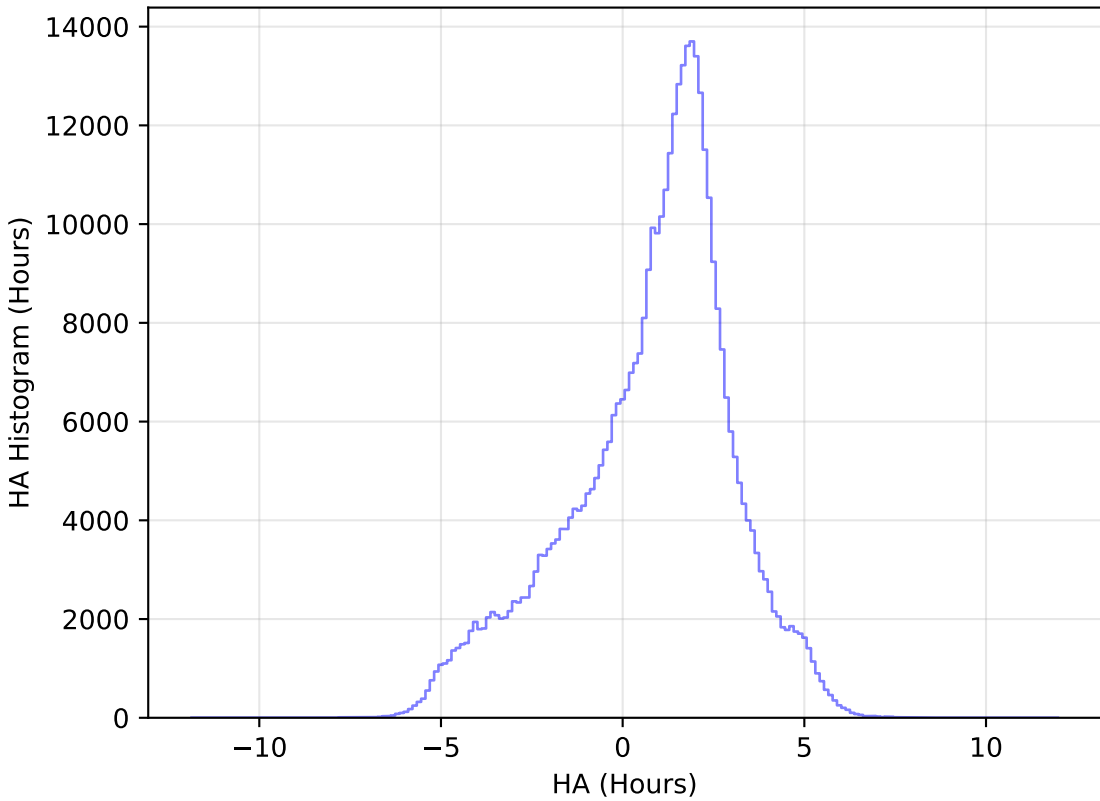
internal_u_expt27_nscale1.0v3.4_10yrs WFD z band: HA Histogram
