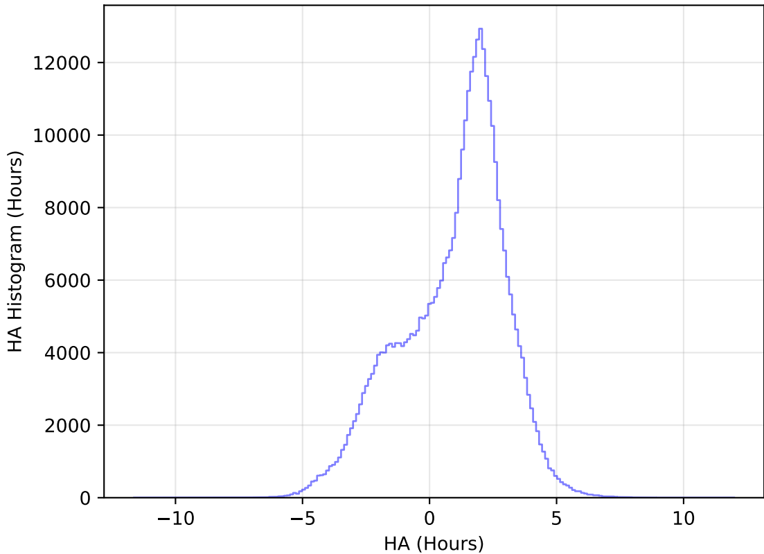
internal_u_expt27_nscale1.0v3.4_10yrs WFD y band: HA Histogram
