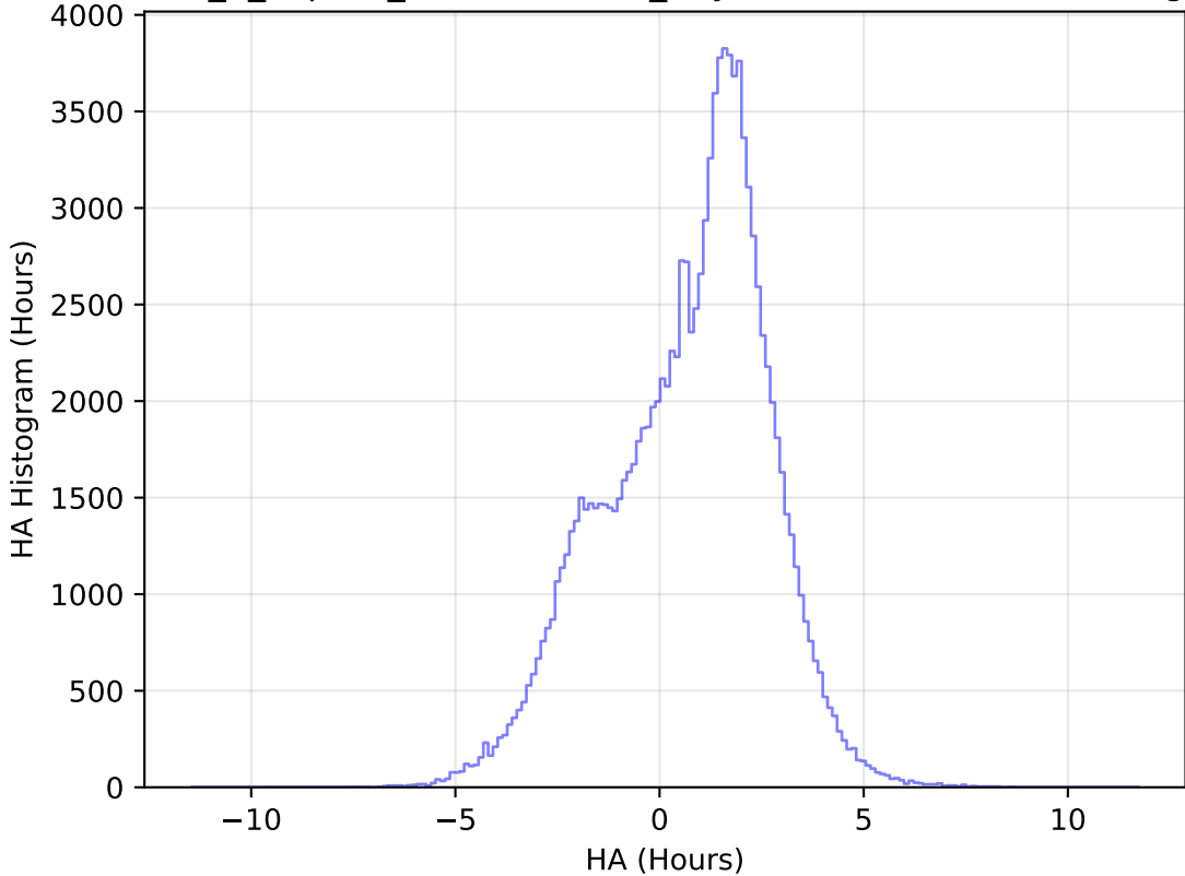
internal_u_expt27_nscale1.0v3.4_10yrs WFD u band: HA Histogram
