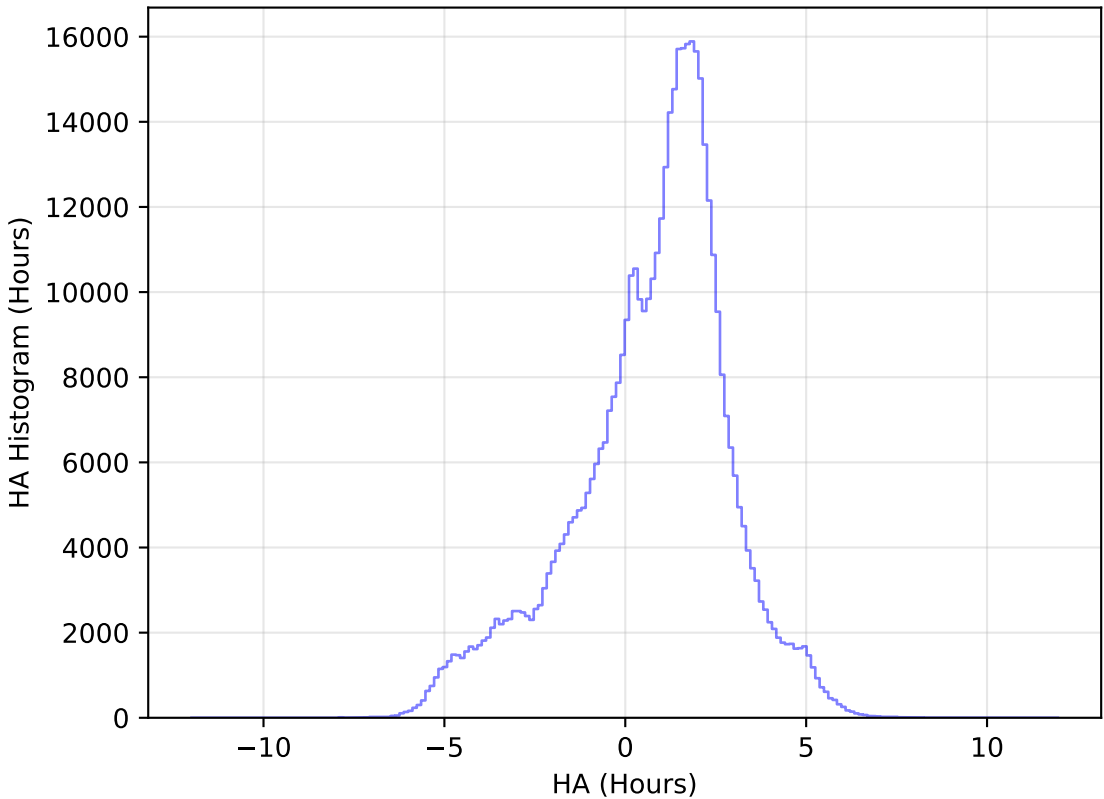
internal_u_expt27_nscale1.0v3.4_10yrs WFD i band: HA Histogram
