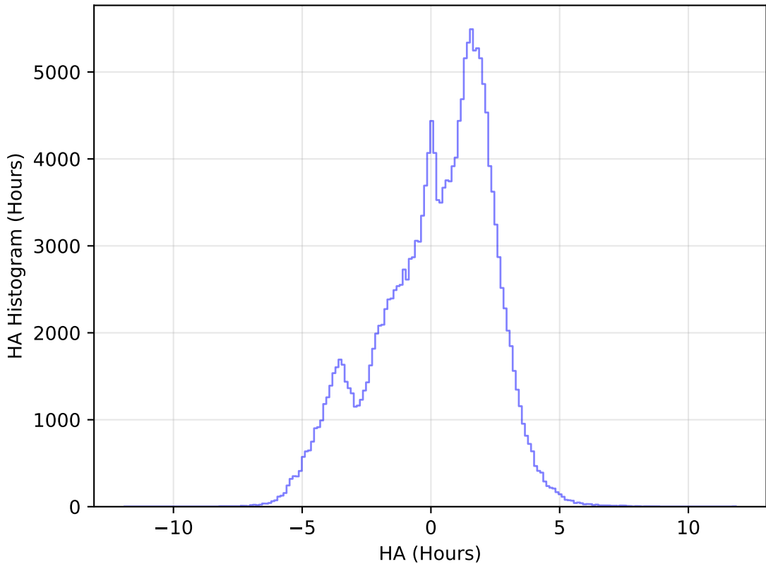
internal_u_expt27_nscale1.0v3.4_10yrs WFD g band: HA Histogram
