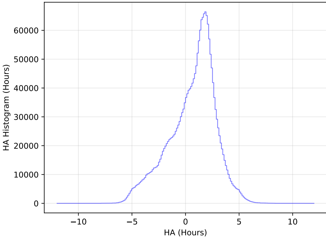
internal_u_expt27_nscale1.0v3.4_10yrs WFD all bands: HA Histogram
