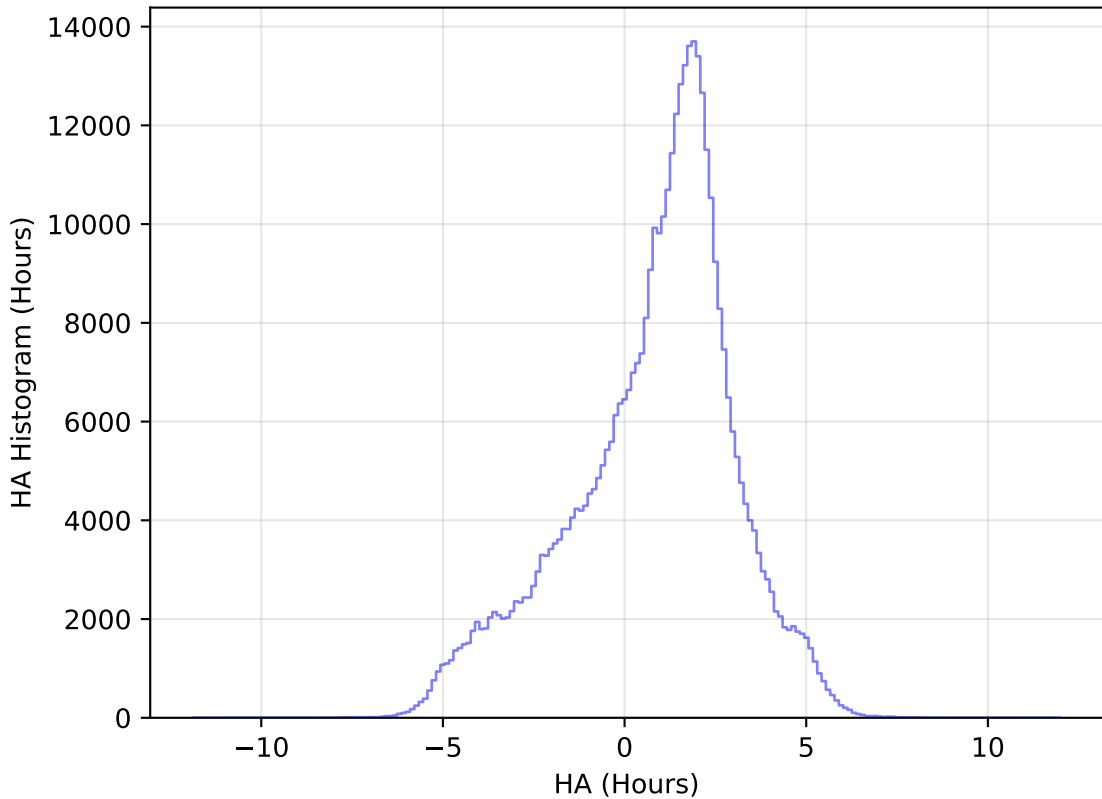
internal_u_expt27_nscale1.0v3.4_10yrs All sky z band: HA Histogram
