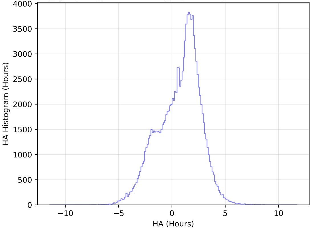
internal_u_expt27_nscale1.0v3.4_10yrs All sky u band: HA Histogram
