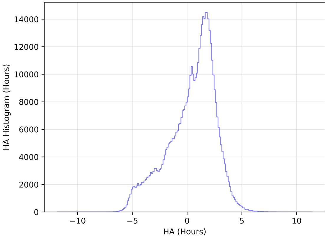
internal_u_expt27_nscale1.0v3.4_10yrs All sky r band: HA Histogram
