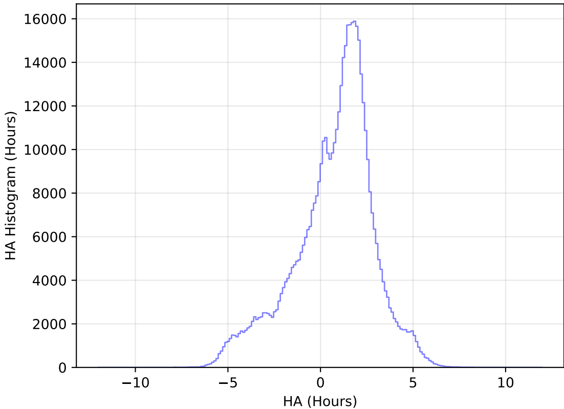
internal_u_expt27_nscale1.0v3.4_10yrs All sky i band: HA Histogram
