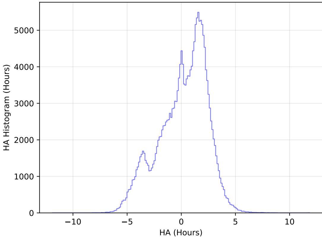
internal_u_expt27_nscale1.0v3.4_10yrs All sky g band: HA Histogram
