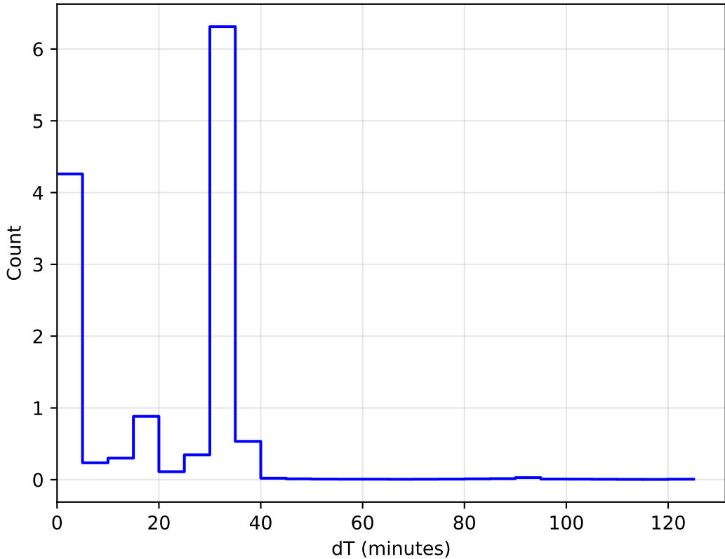
internal_u_expt27_nscale1.0v3.4_10yrs All sky: DeltaT Histogram 1e6
