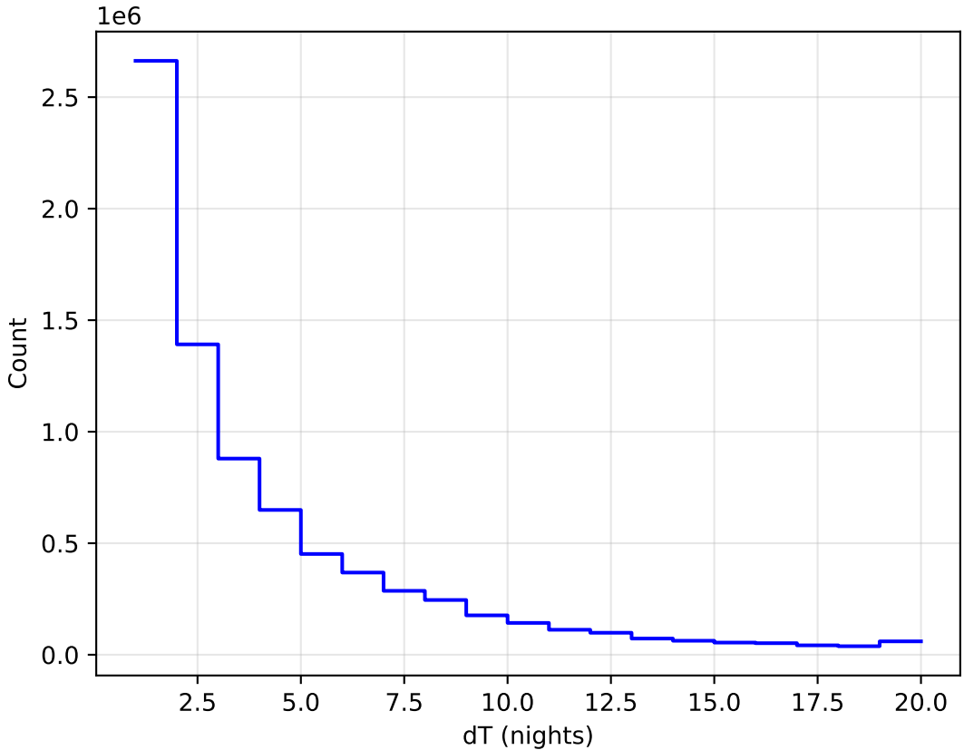
internal_u_expt27_nscale1.0v3.4_10yrs WFD all bands: DeltaNight Histogram
