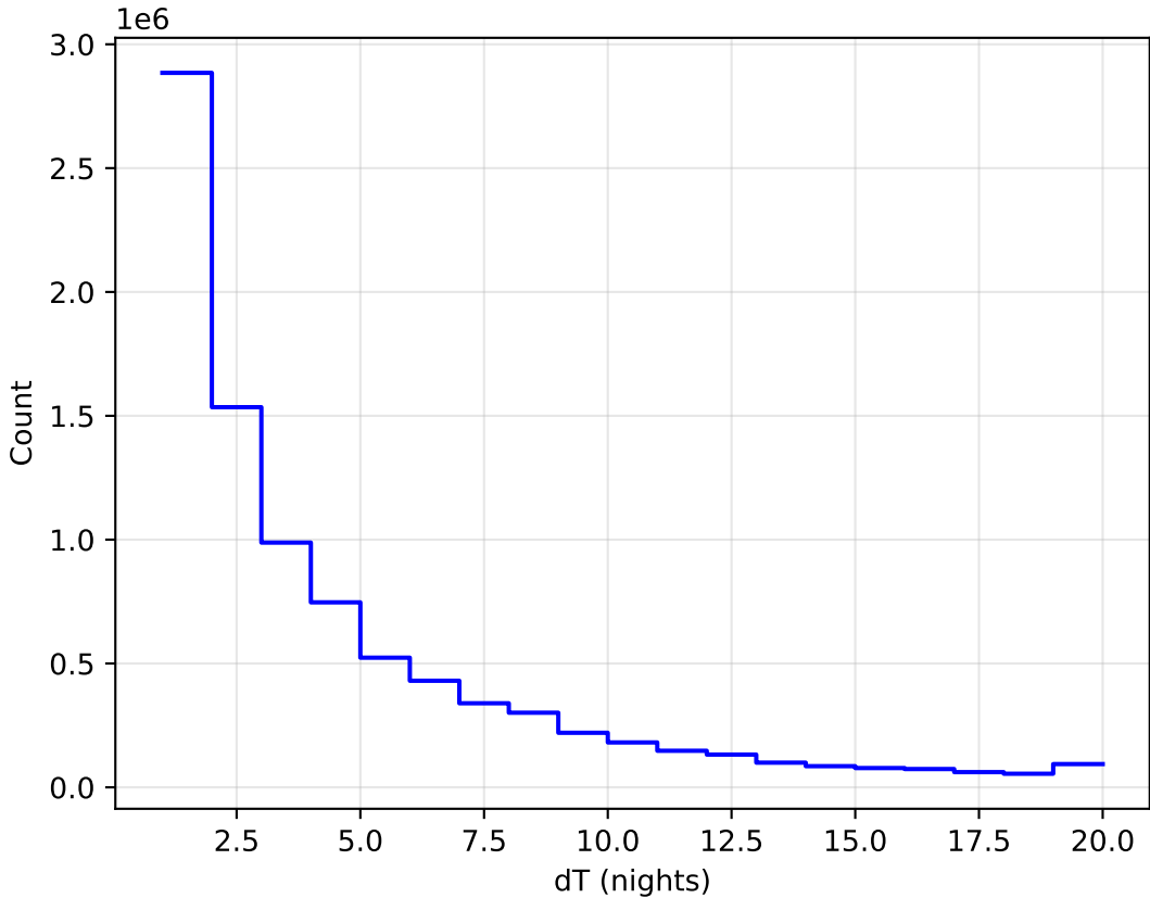
internal_u_expt27_nscale1.0v3.4_10yrs All sky all bands: DeltaNight Histogram
