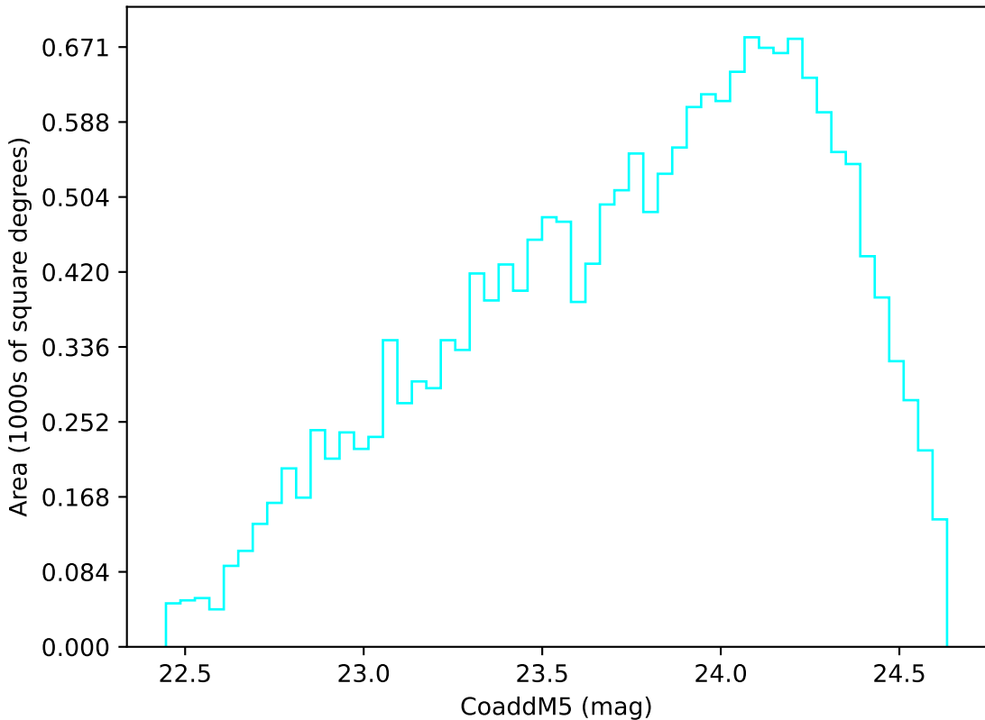
internal_u_expt27_nscale1.0v3.4_10yrs Yr 3-4 u band: CoaddM5
