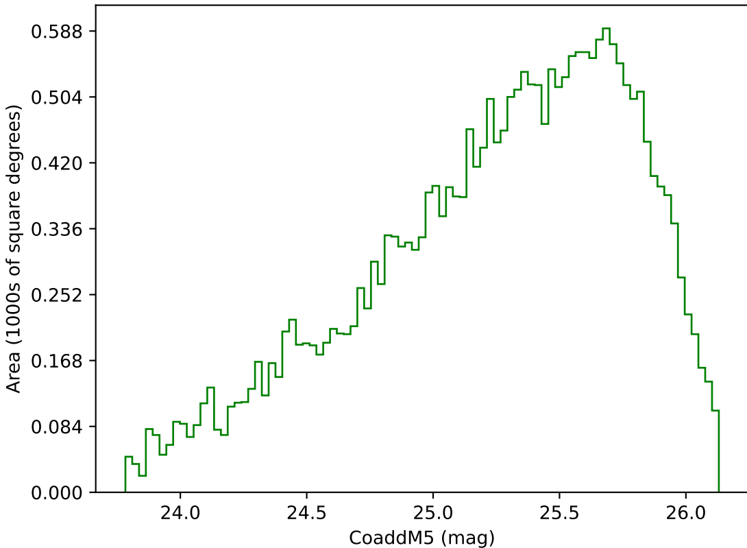
internal_u_expt27_nscale1.0v3.4_10yrs Yr 3-4 g band: CoaddM5
