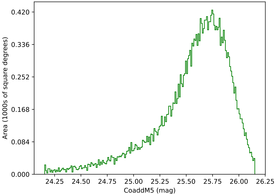
internal_u_expt27_nscale1.0v3.4_10yrs Yr 1 g band: CoaddM5
