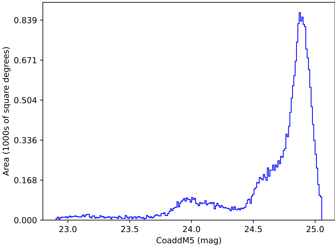
internal_u_expt27_nscale1.0v3.4_10yrs All sky y band: CoaddM5
