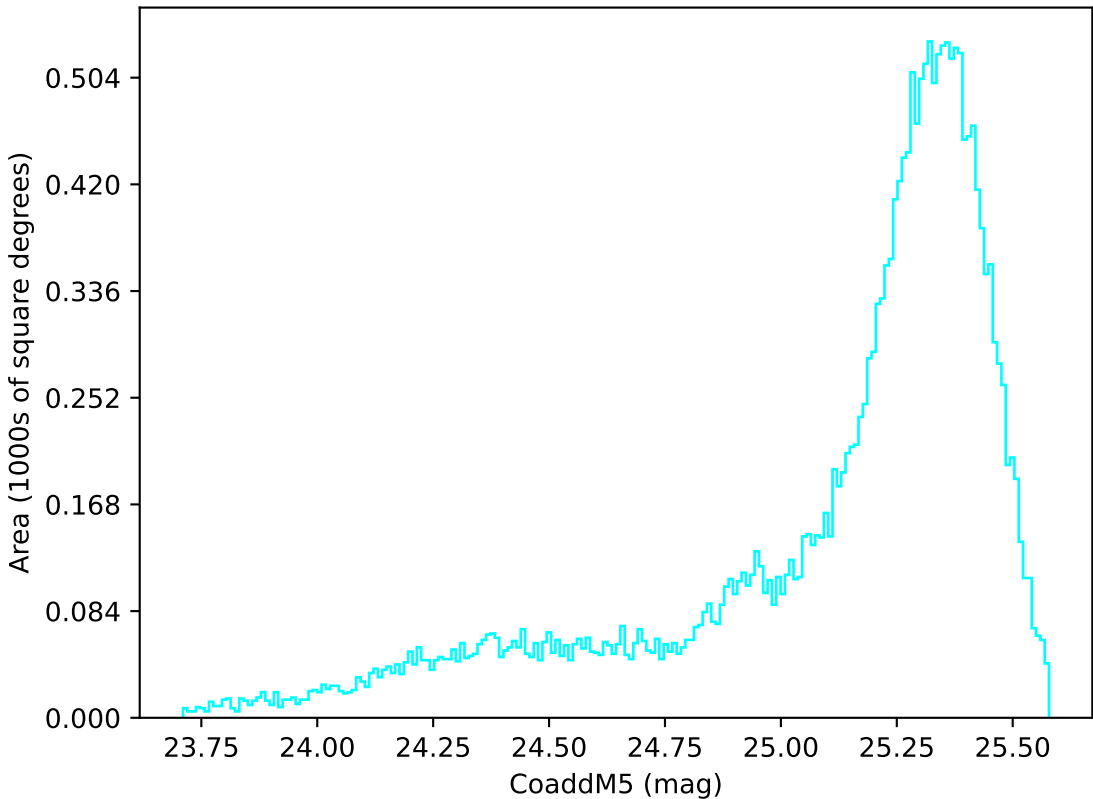
internal_u_expt27_nscale1.0v3.4_10yrs All sky u band: CoaddM5
