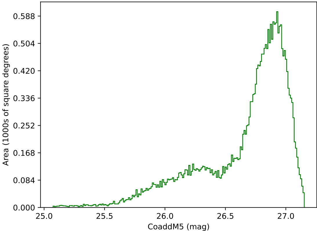
internal_u_expt27_nscale1.0v3.4_10yrs All sky g band: CoaddM5
