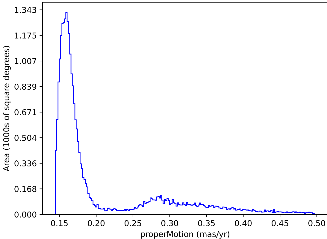
internal_u_expt27_nscale1.0v3.4_10yrs : properMotion
