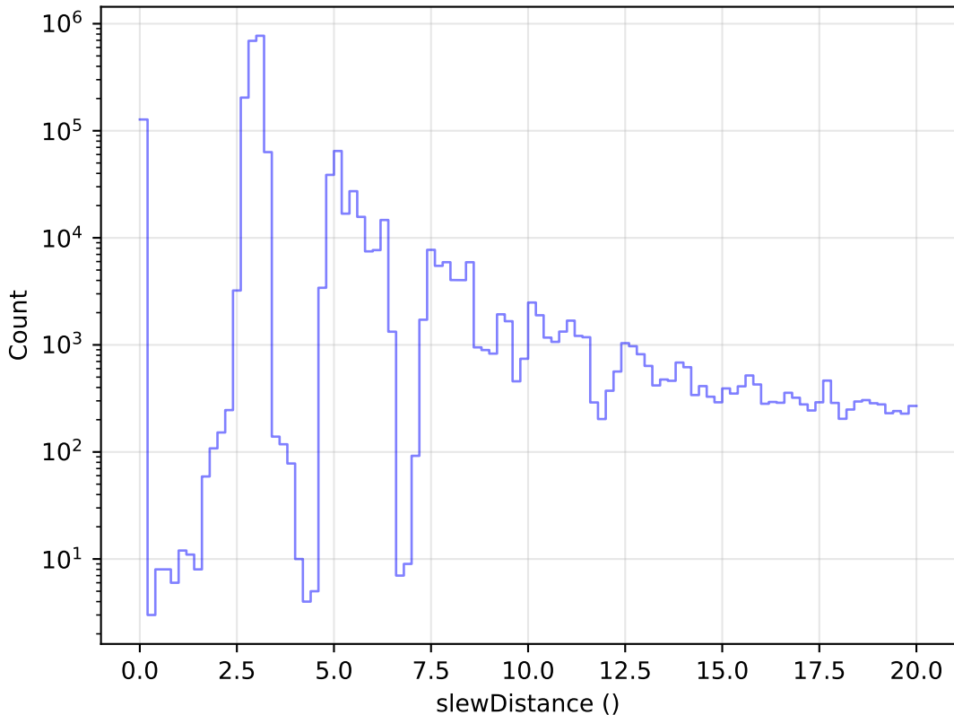
internal_u_expt27_nscale1.0v3.4_10yrs All visits: Zoom Slew Distance Histogram
