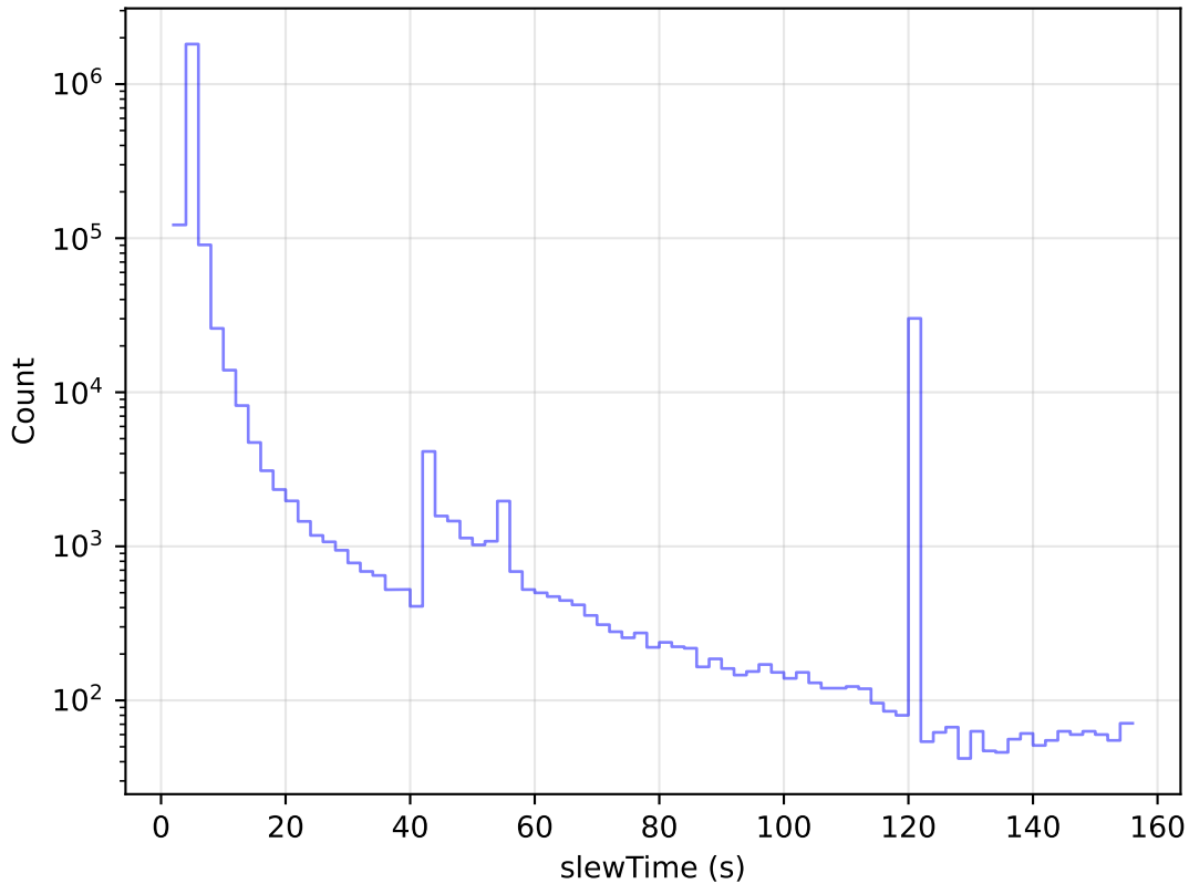
internal_u_expt27_nscale1.0v3.4_10yrs All visits: Slew Time Histogram
