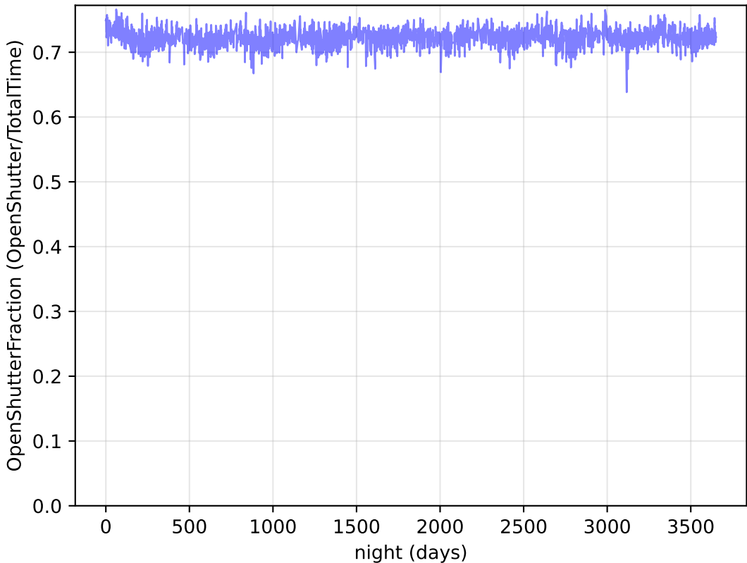
internal_u_expt27_nscale1.0v3.4_10yrs : OpenShutterFraction
