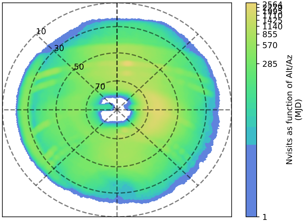
internal_u_expt27_nscale1.0v3.4_10yrs r: Nvisits as function of Alt/Az
