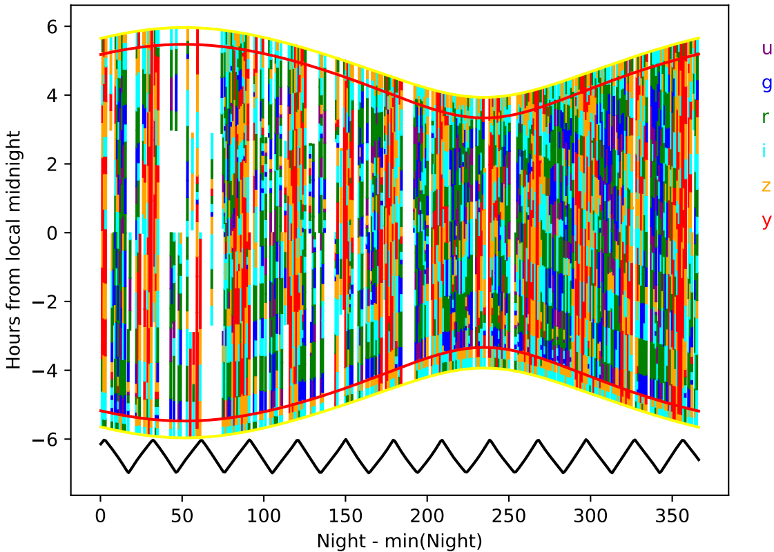
internal_u_expt27_nscale1.0v3.4_10yrs year 9-10: Hourglass
