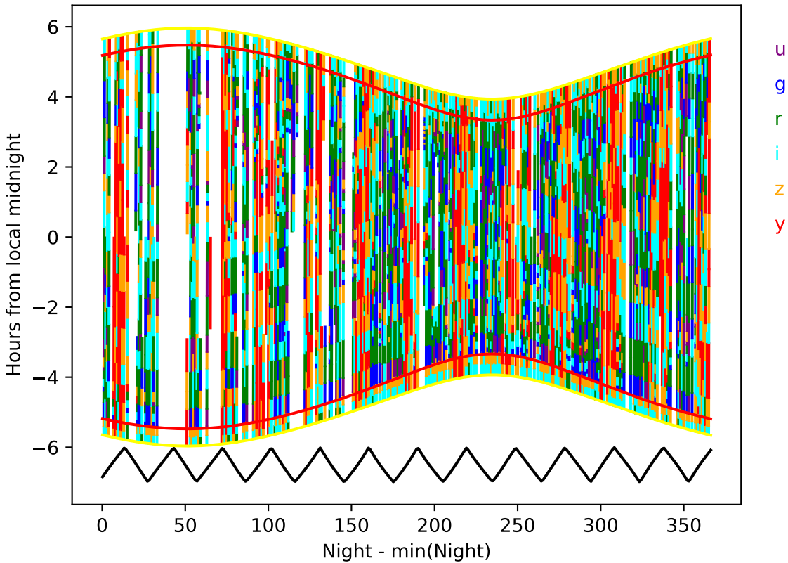
internal_u_expt27_nscale1.0v3.4_10yrs year 8-9: Hourglass
