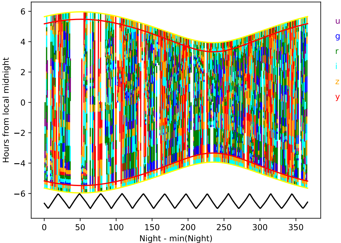
internal_u_expt27_nscale1.0v3.4_10yrs year 2-3: Hourglass
