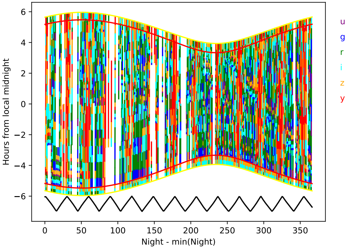
internal_u_expt27_nscale1.0v3.4_10yrs year 1-2: Hourglass
