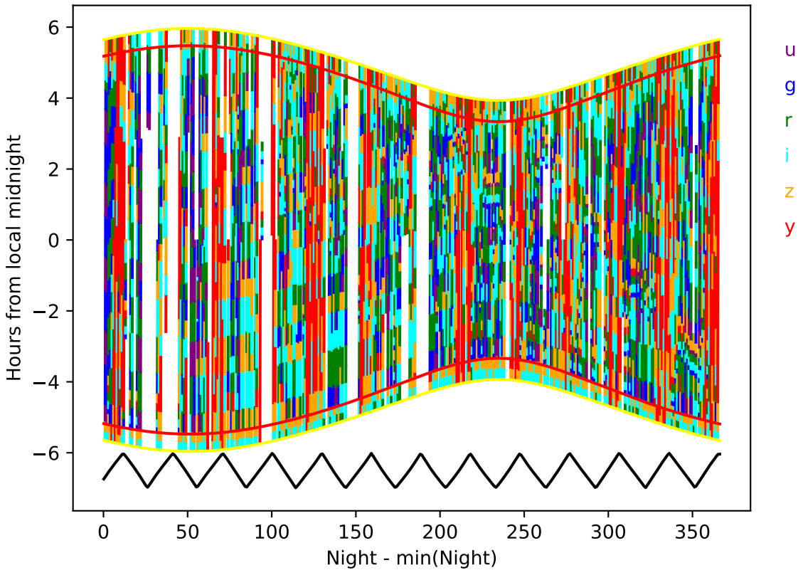
internal_u_expt27_nscale1.0v3.4_10yrs year 0-1: Hourglass
