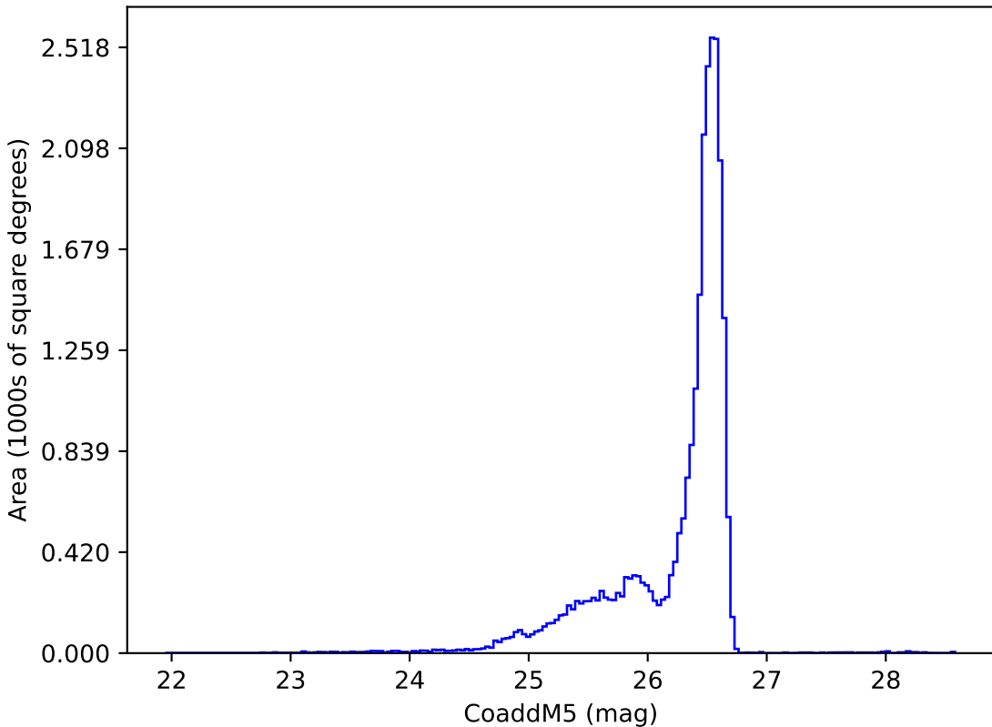
internal_u_expt27_nscale1.0v3.4_10yrs i: CoaddM5
