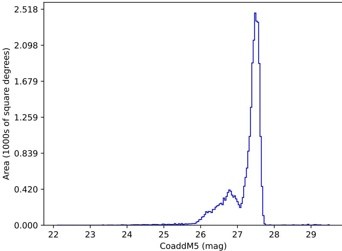
internal_u_expt27_nscale1.0v3.4_10yrs : CoaddM5
