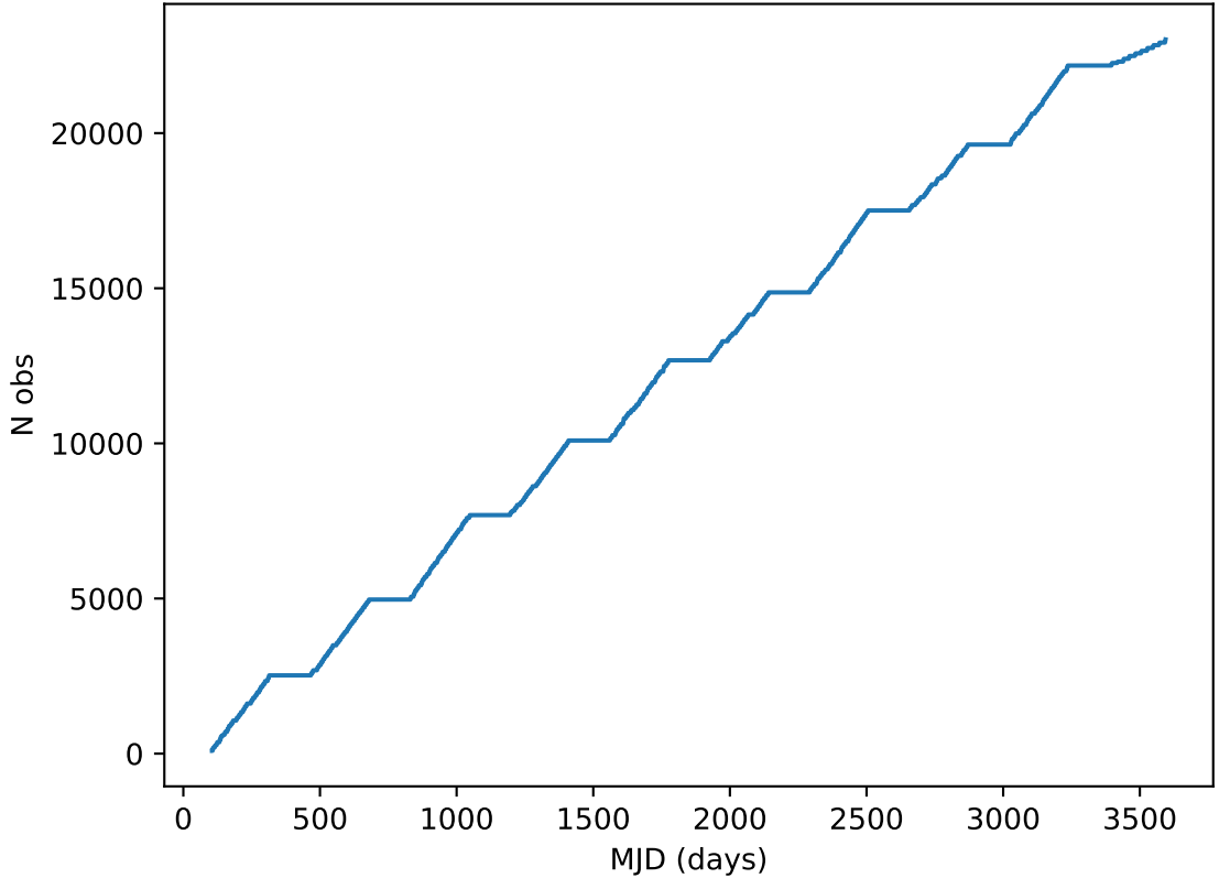
internal_u_expt27_nscale1.0v3.4_10yrs all bands: DD:EDFS Cumulative NVisits
