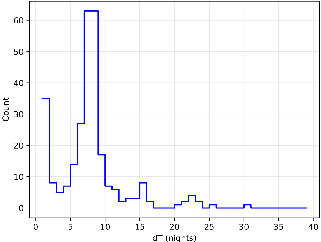
internal_u_expt27_nscale1.0v3.4_10yrs all bands: DD:ECDFS Delta Nights Histogram
