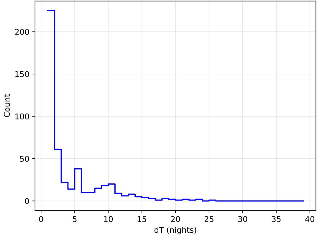
internal_u_expt27_nscale1.0v3.4_10yrs all bands: DD:COSMOS Delta Nights Histogram
