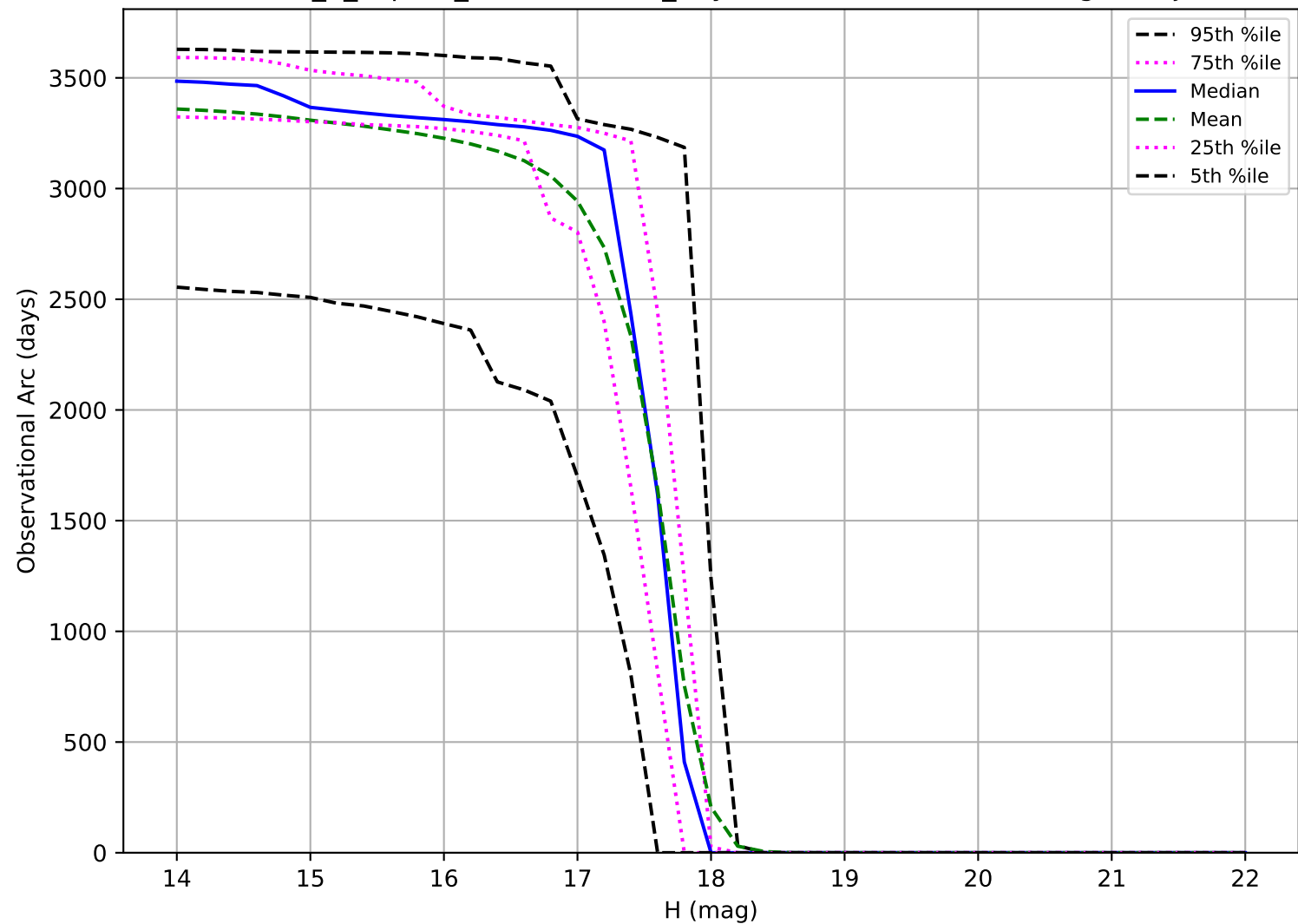
internal_u_expt27_nscale0.9v3.4_10yrs: Observational Arc Length Trojan
