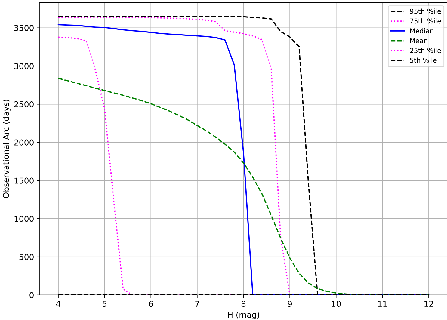
internal_u_expt27_nscale0.9v3.4_10yrs: Observational Arc Length TNO
