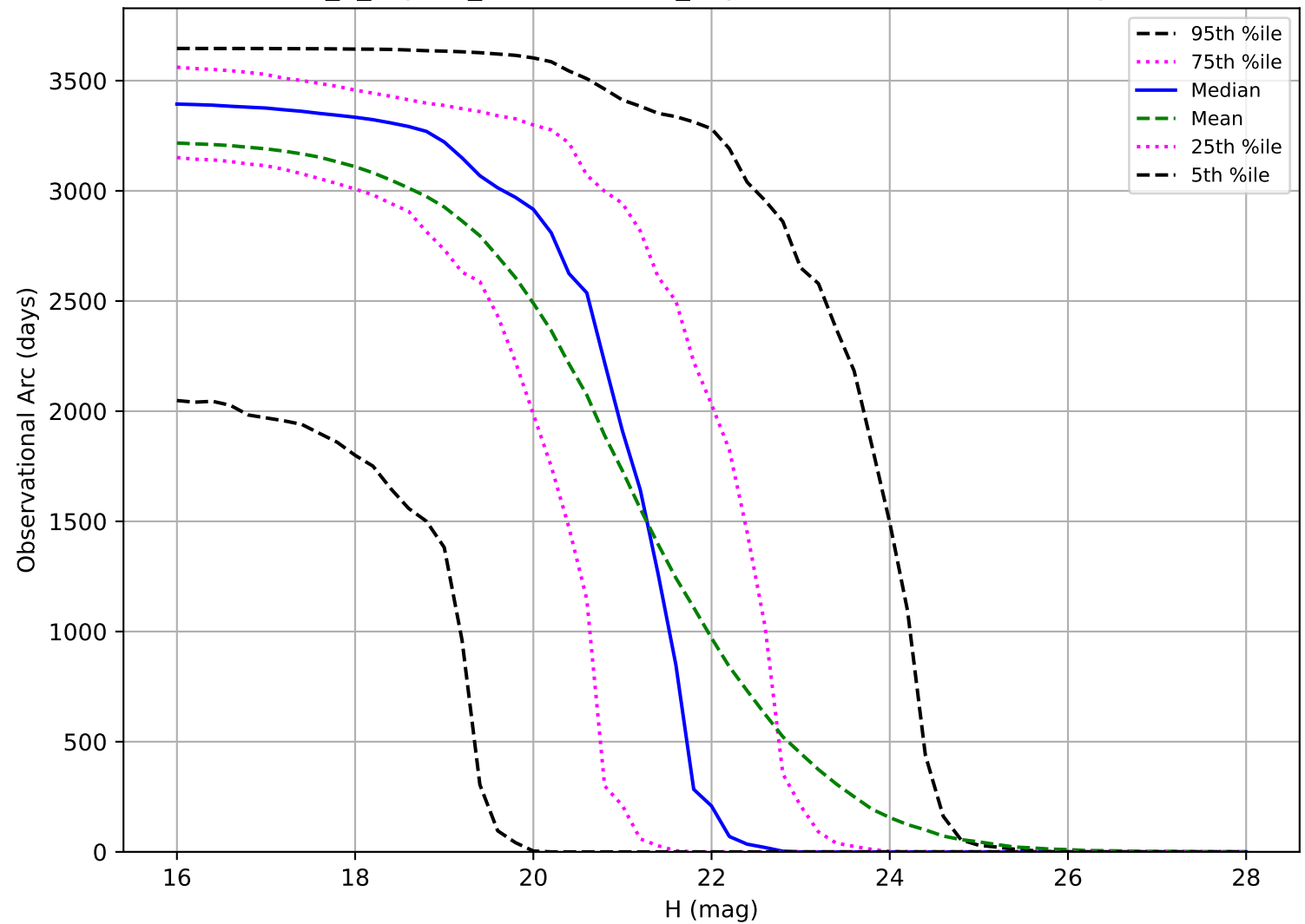
internal_u_expt27_nscale0.9v3.4_10yrs: Observational Arc Length PHA
