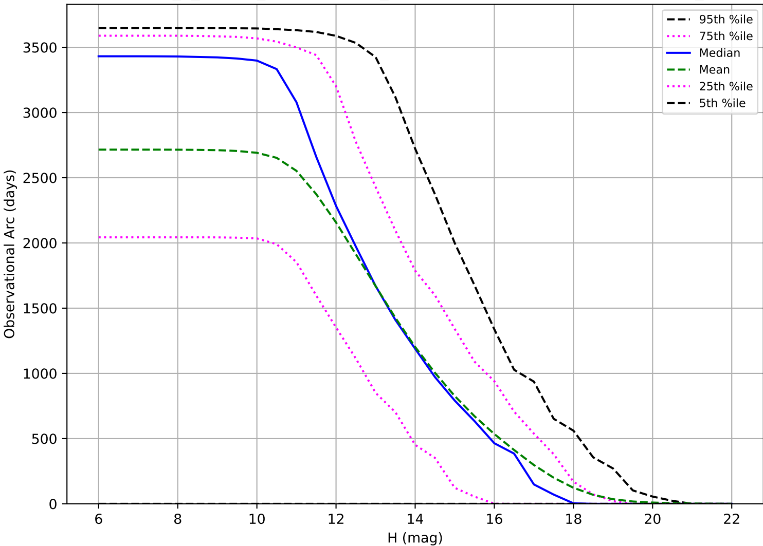
internal_u_expt27_nscale0.9v3.4_10yrs: Observational Arc Length OCC_r5
