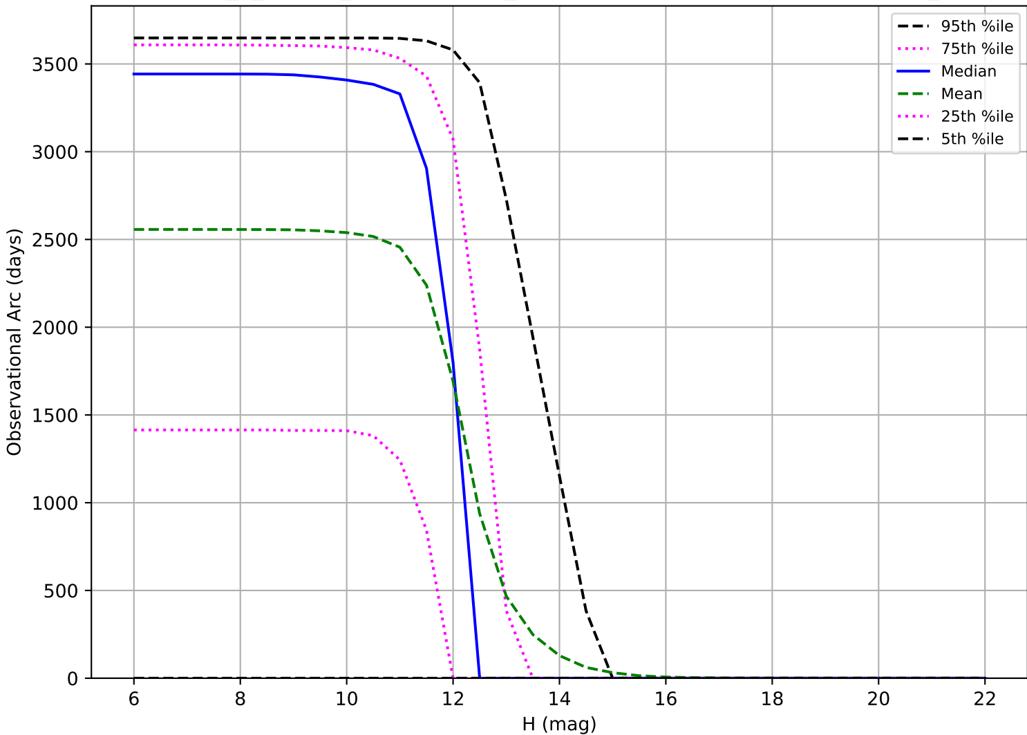
internal_u_expt27_nscale0.9v3.4_10yrs: Observational Arc Length OCC_r20
