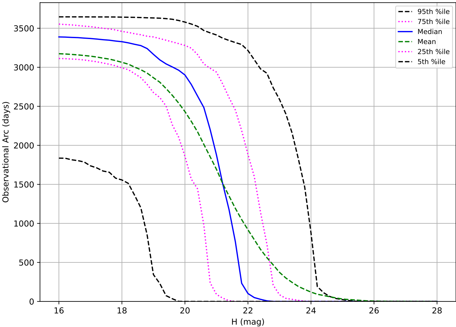
internal_u_expt27_nscale0.9v3.4_10yrs: Observational Arc Length NEO
