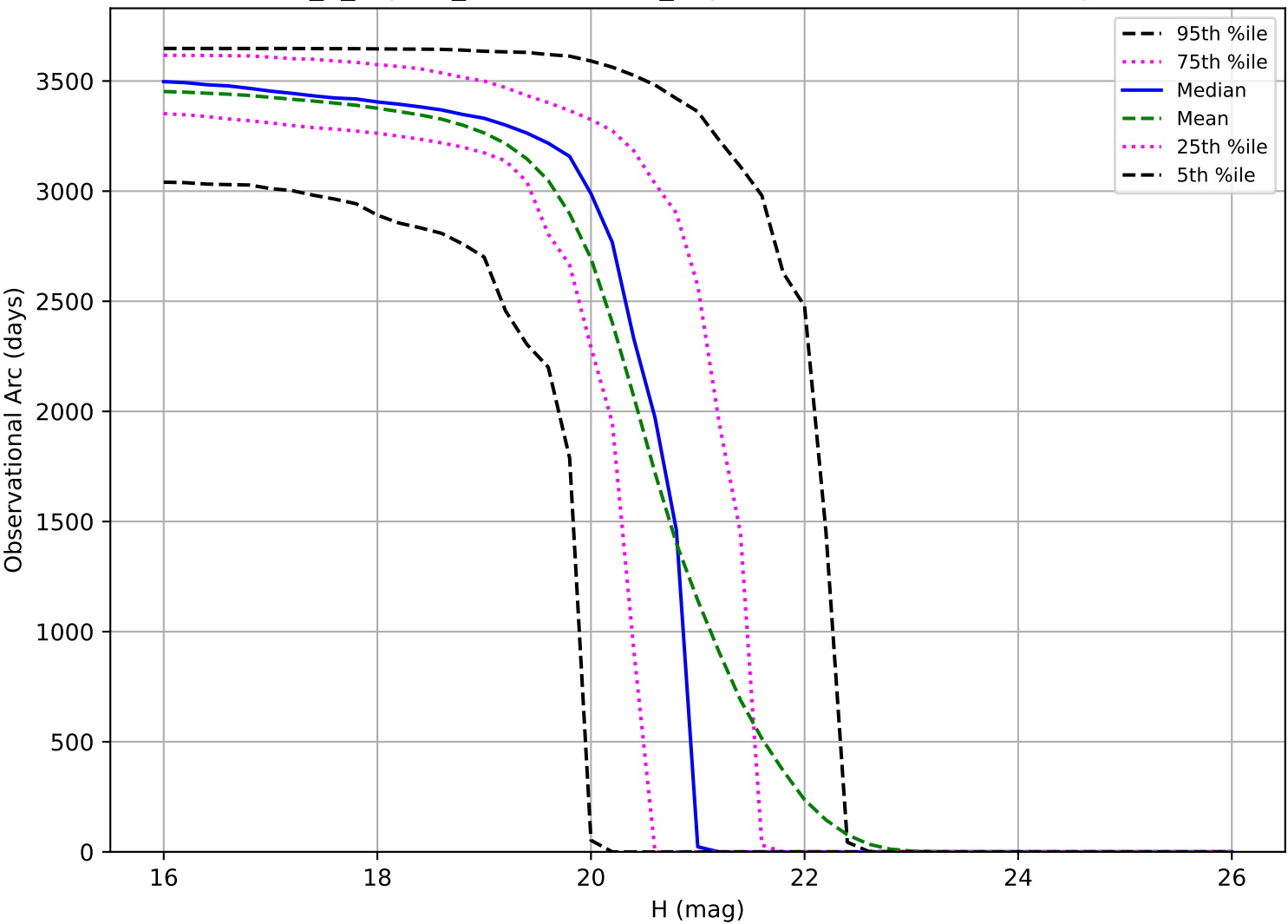
internal_u_expt27_nscale0.9v3.4_10yrs: Observational Arc Length MBA
