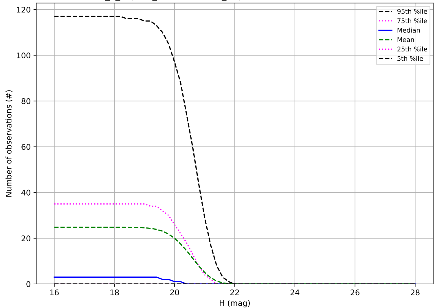
internal_u_expt27_nscale0.9v3.4_10yrs: Number of observations Vatira
